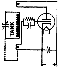
Meissner oscillator circuit.
